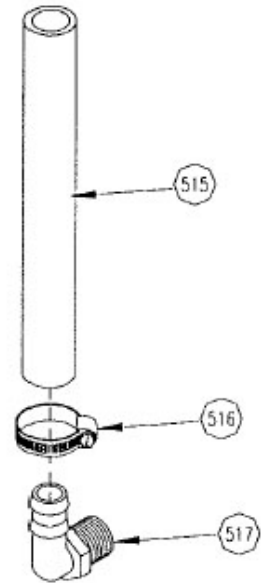
FOAM DROP COUPLER ASSEMBLY
